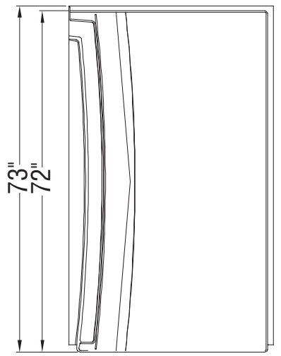
Wall B
