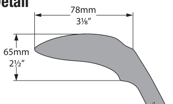
Rim Detail
